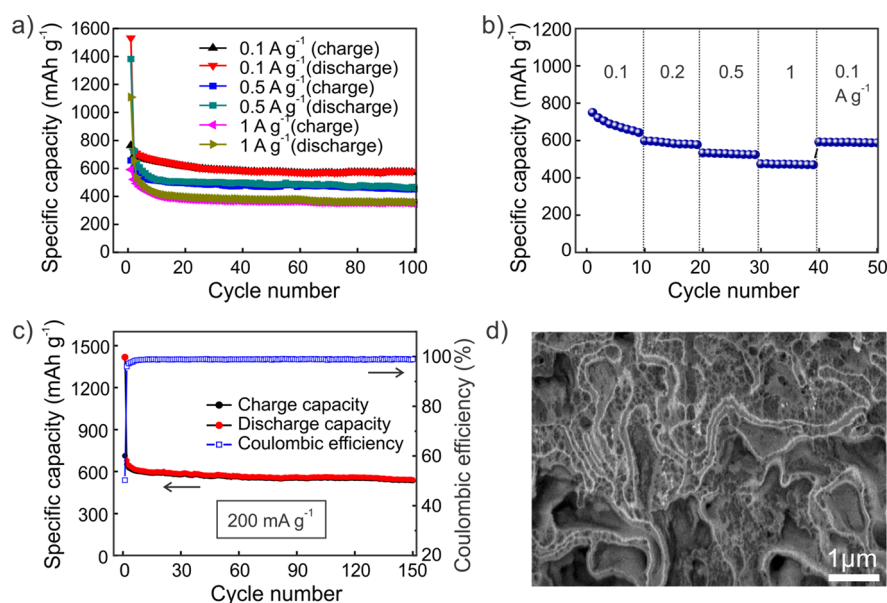
Figure 5. Electrochemical characterization of the sandwich-stacked \text{SnO}_2/\text{Cu} nanosheets as anodes in lithium ion batteries: (a) comparative cycling performance showing the discharge and charge capacities of the sandwich-stacked \text{SnO}_2/\text{Cu} nanosheets at current rates of 100, 500, and 1000 \text{mA g}^{-1} ; (b) rate capability of the stacked \text{SnO}_2/\text{Cu} nanosheets; (c) cycling performance for 150 cycles at a current rate of 200 \text{mA g}^{-1} from 0.05 to 1.5 V versus \text{Li}/\text{Li}^+ ; (d) electron backscattering contrast on cross-sectional image of the stacked \text{SnO}_2/\text{Cu} nanosheets at a fully charged state after 100 cycles.
